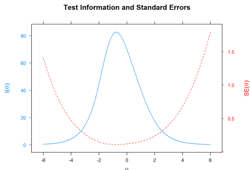
Figur 2: Test Information and Standard errors
